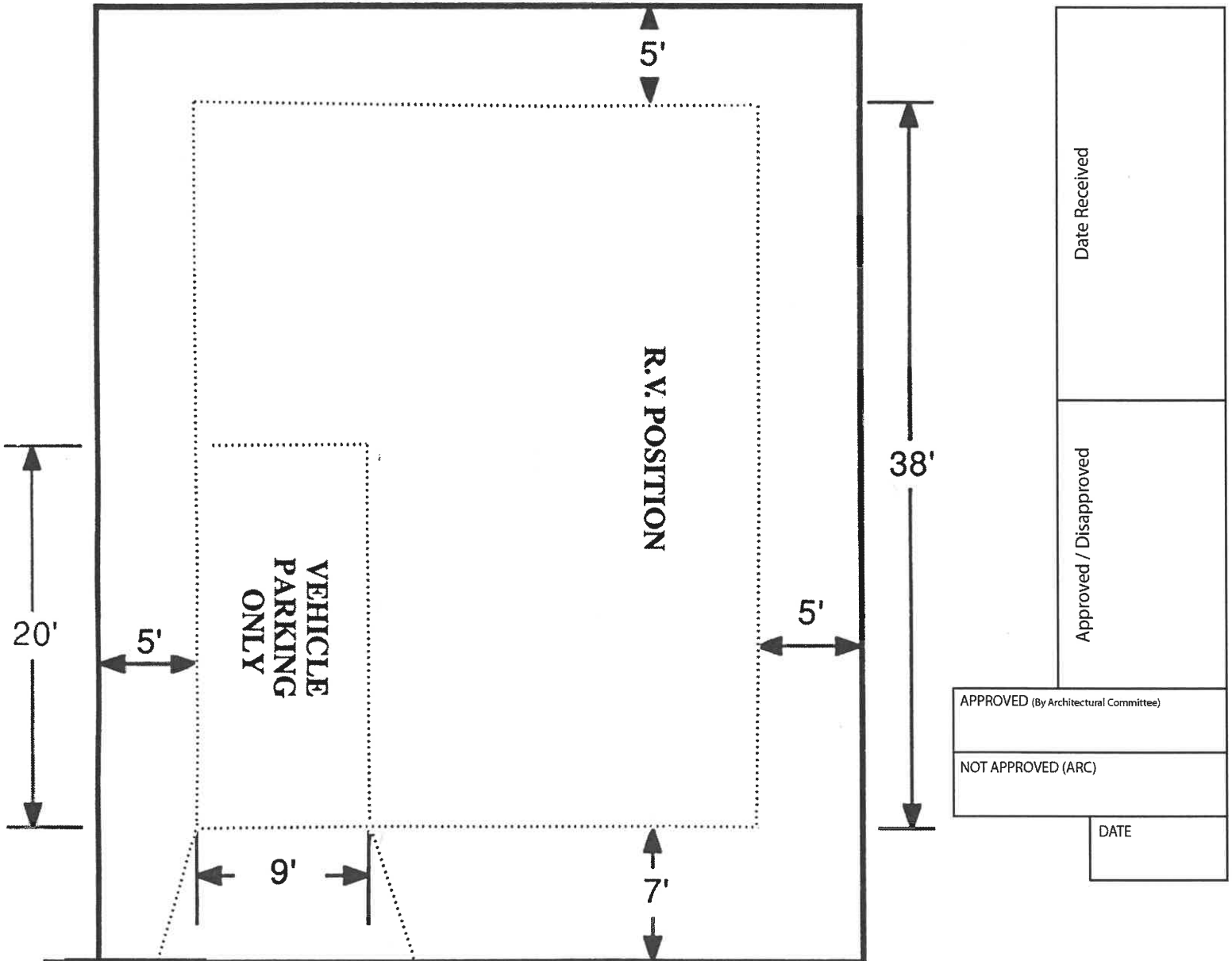
DRAWING OF TYPICAL LOT SHOWING LOCATION OF CONSTRUCTION
